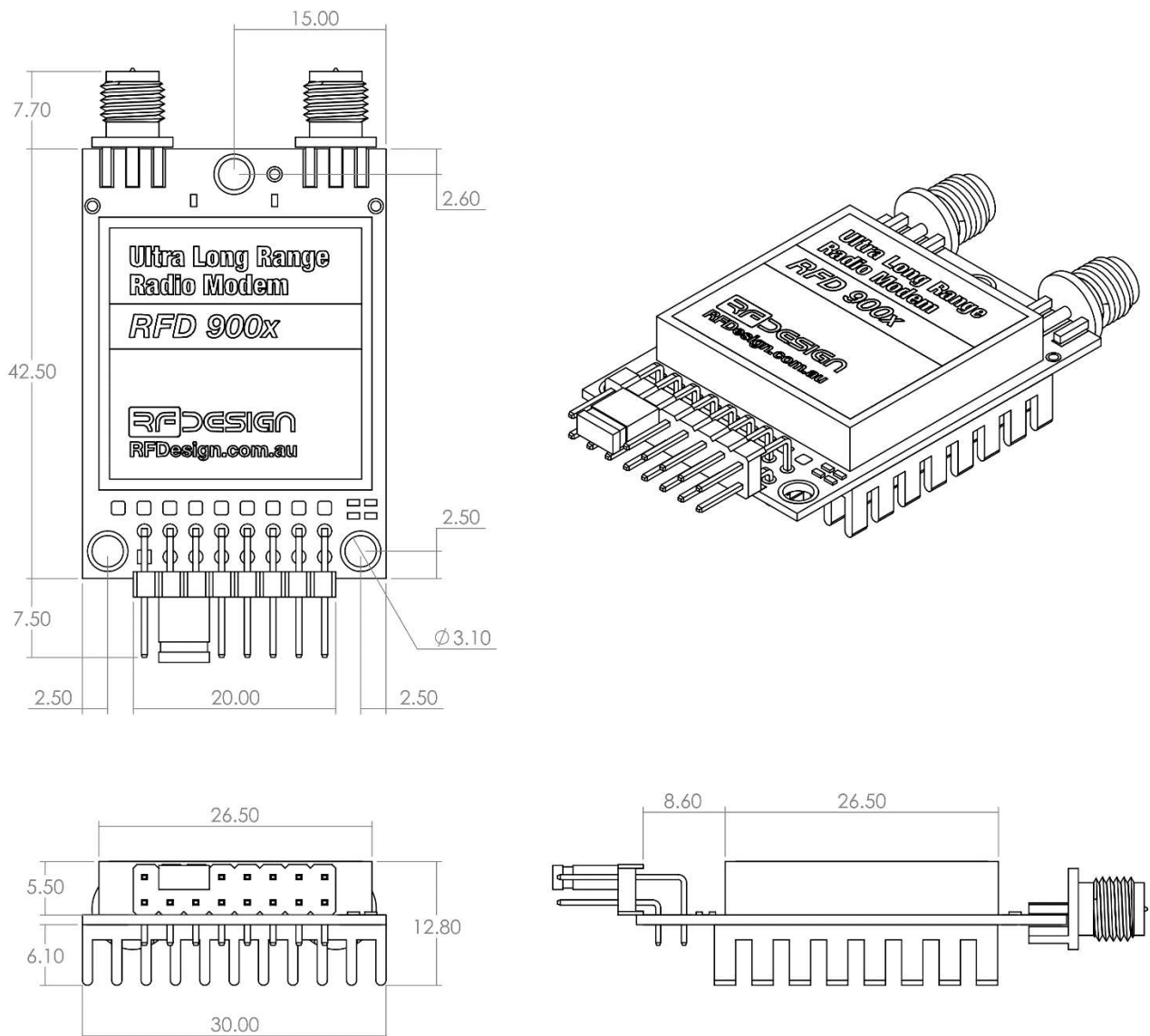
Figure 38: x series modem dimension drawing
